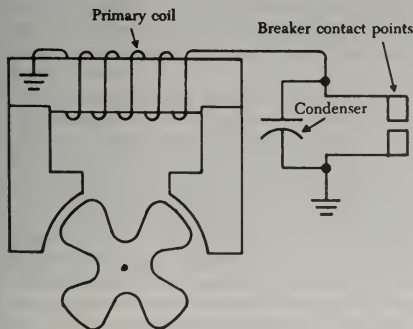
FIGURE 4-4. Primary electrical circuit of a high-tension magneto.
